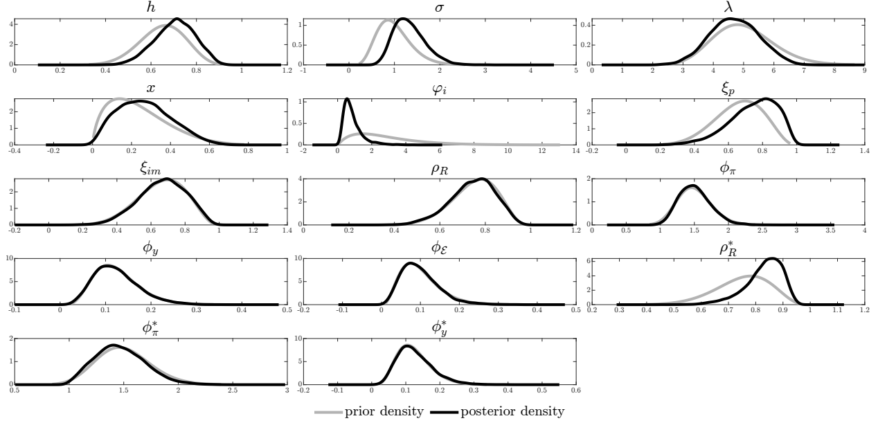
Figure A.9: Prior and posterior densities for impulse response matching exercise
